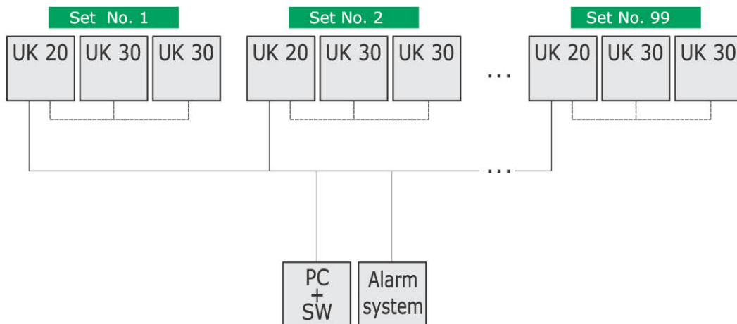
Figure 5 - Block diagram showing the connection of key deposit case sets
